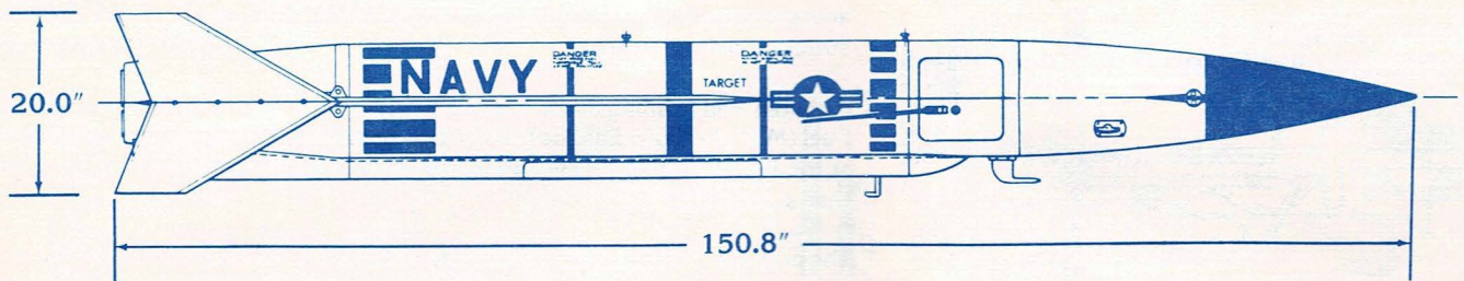
SIDE VIEW
