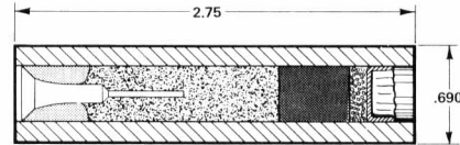
PORT BURNING
