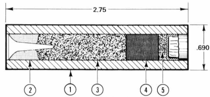
END BURNING
