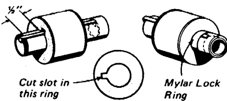
Adapting an engine lock to an EM-13, 16, 20 engine mount
