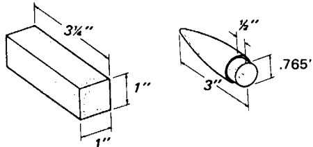
Experimental Fin
