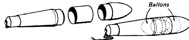
Centuri's Egg Capsule (No. PNC-13E/ST-202)
