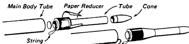
Centuri's Egg Capsule (No. PNC-13E/ST-202)
