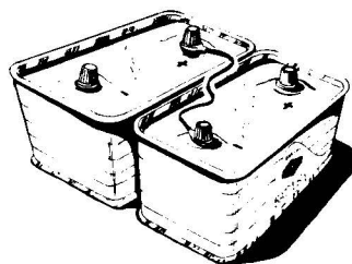
Two 6 Volt Lantern Batteries Combined in Series. This now produces a total of 12 Volts.
