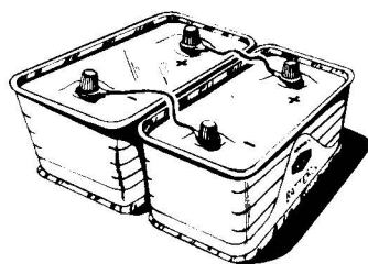
Two 6 Volt Lantern Batteries Combined in Parallel. This Still Produces 6 Volts.
