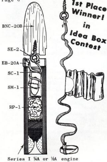
Series I \frac{1}{4} A or \frac{1}{2} A engine
