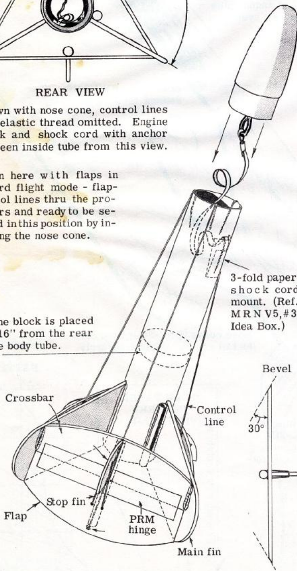
FLAP DETAIL
