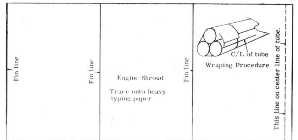
Fin Root & Tip Pattern (BFS-40)
